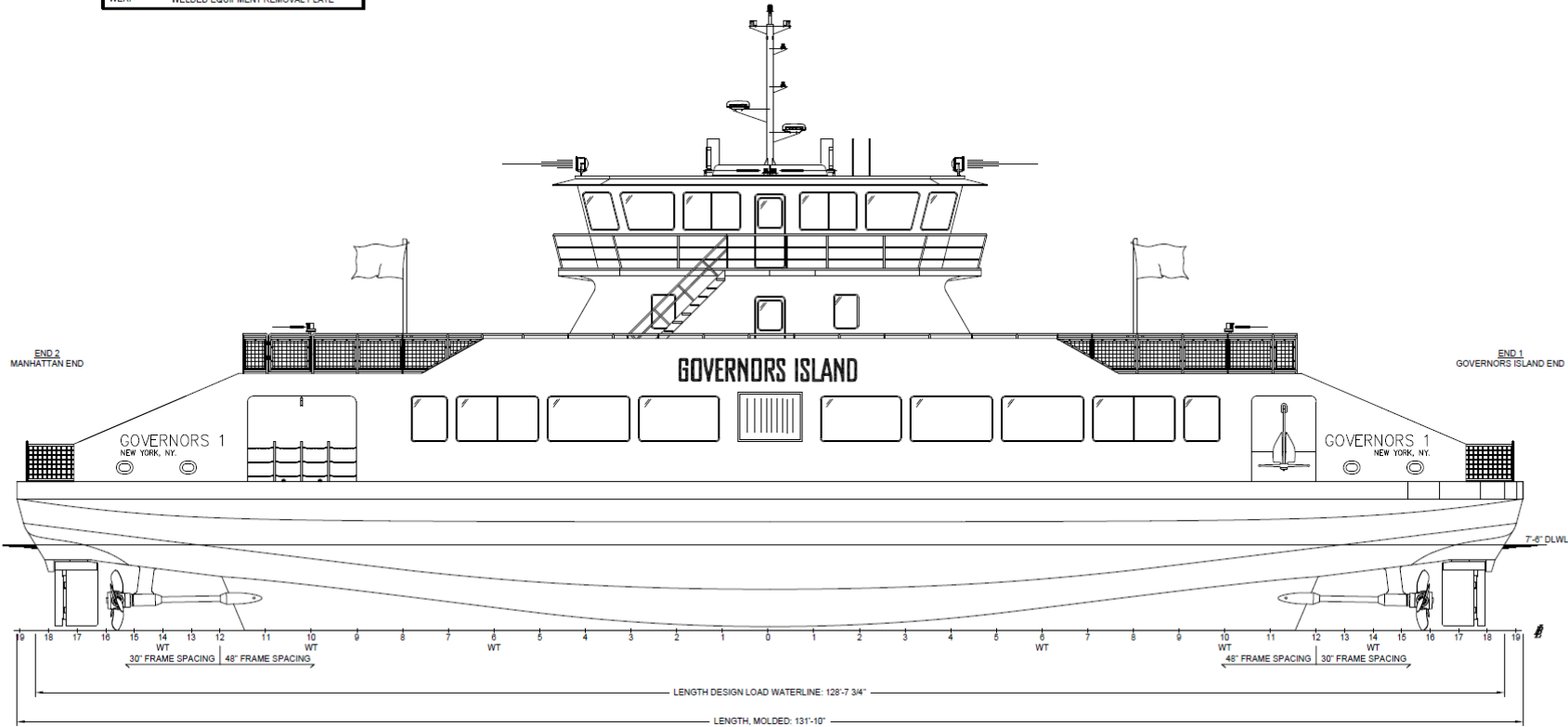
PROFILE 1-5A OUTBOARD PROFILE 3/16"=1'-0"
